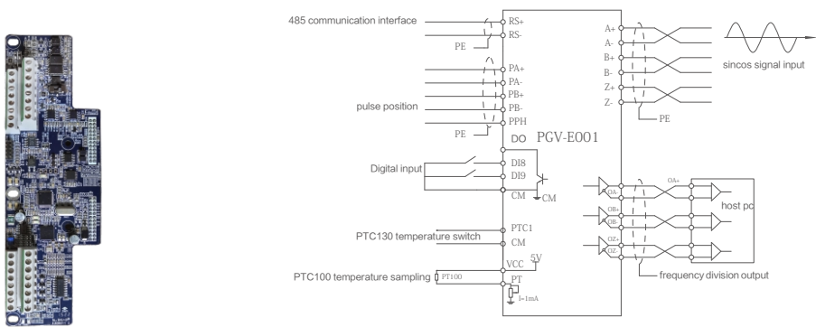
Wiring Diagram of sine and cosine PG card
