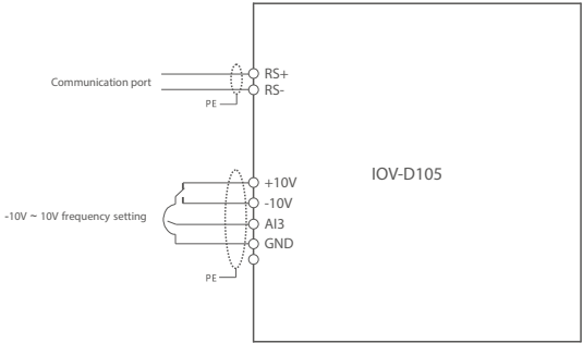
Communication Card Wiring Diagram
