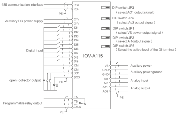
I/O Extension Card Wiring Diagram
