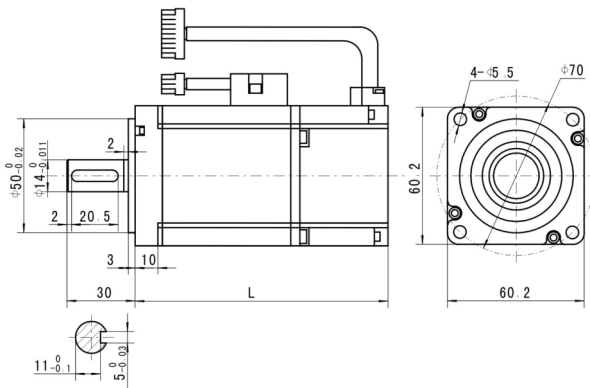
60 Flange Motor Dimension
