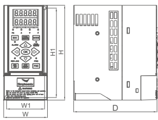
Mounting dimension
