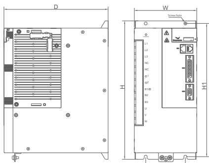
II Class applicable models: CA100-F20RAP~CA100-F25RAP
