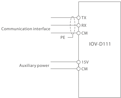
Extension Card Wiring Diagram
