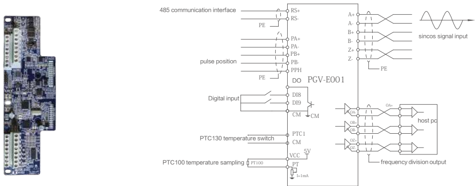
Wiring Diagram of sine and cosine PG card
