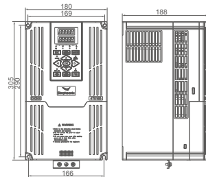
Note: two special models DX500-4T0150G/4T0185PQ DX500-4T0185G/4T0220PQ
