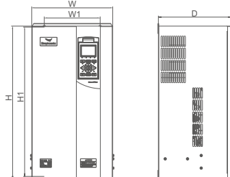
Class IV applicable model: DX500-4T0450G/4T0550PQ~DX500-4T3150G/4T3500PQ
