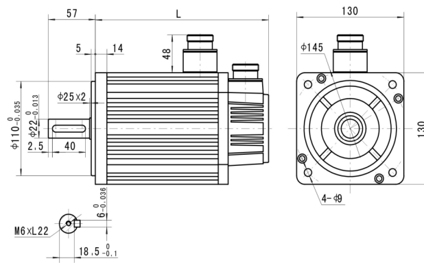
130 Flange Motor Dimension
