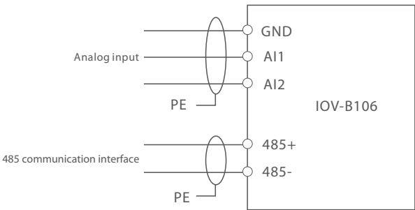
Air compressor communication adapter card wiring diagram
