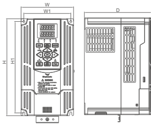
Class III applicable model: DX500-4T0055G/4T0075PQ~ DX500-4T0370G/4T0450PQ
