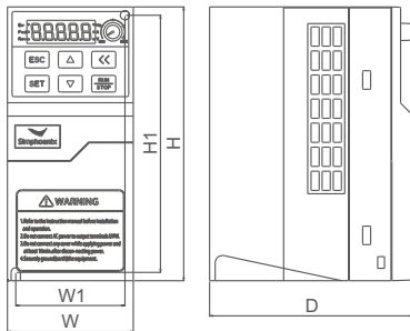
Class I DL300-4T0011GQ ~ DL300-4T0015GQ DL300-2S0007Q ~ 2S0015Q
