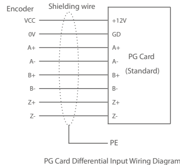
PG Card Differential Input Wiring Diagram
