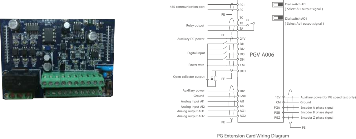
PG Extension Card Wiring Diagram
