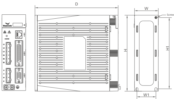
I Class applicable models: CA100-T1R8AP~ CA100-T10RAP CA100-F4R0AP~ CA100-F12RAP
