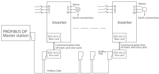
DP Communication Card Wiring Diagram
