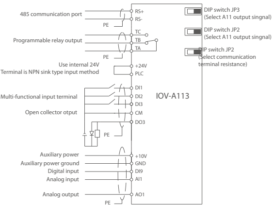
I/O Extension Card Wiring Diagram
