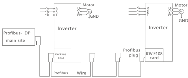
Profibus-DP Communication Card Wiring Diagram
