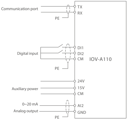
I/O Extension Card Wiring Diagram
