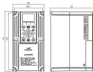
Class II applicable model: DX500-2S0007Q~DX500-2S0022Q DX500-4T0015G/4T0022PQ~DX500-4T0040G/4T0055PQ
