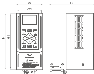
Class I applicable model: DX500-4T0011G/4T0015PQ
