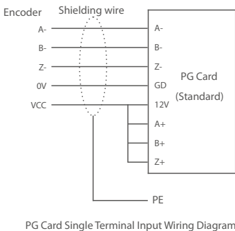
PG Card Single Terminal Input Wiring Diagram
