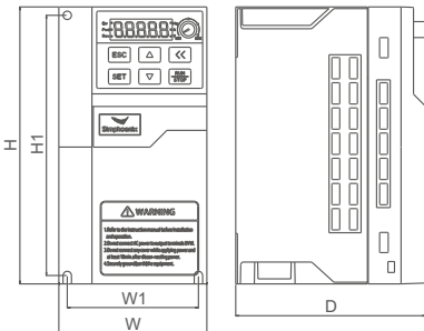
Class II III and IV DL300-4T0022GQ ~ DL300-4T0150GQ DL300-2S0022Q ~ 2S0040Q
