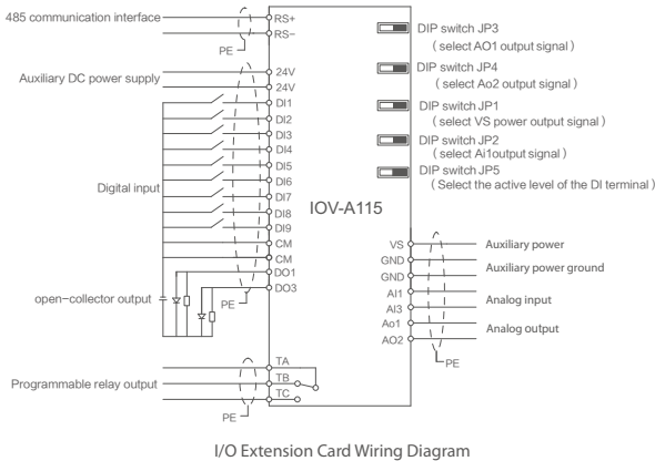
I/O Extension Card Wiring Diagram
